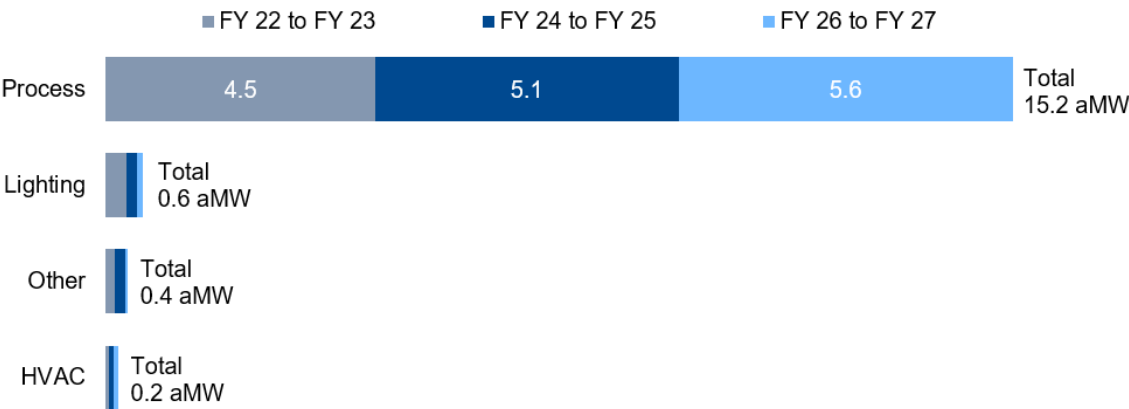
Figure 27. Federal Energy Savings Forecast by End Use and Rate Period
