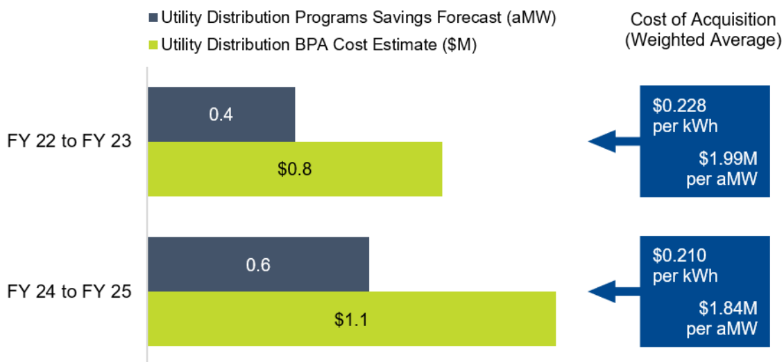
Figure 34. Utility Distribution Program Energy Savings and Cost Metrics by Rate Period
