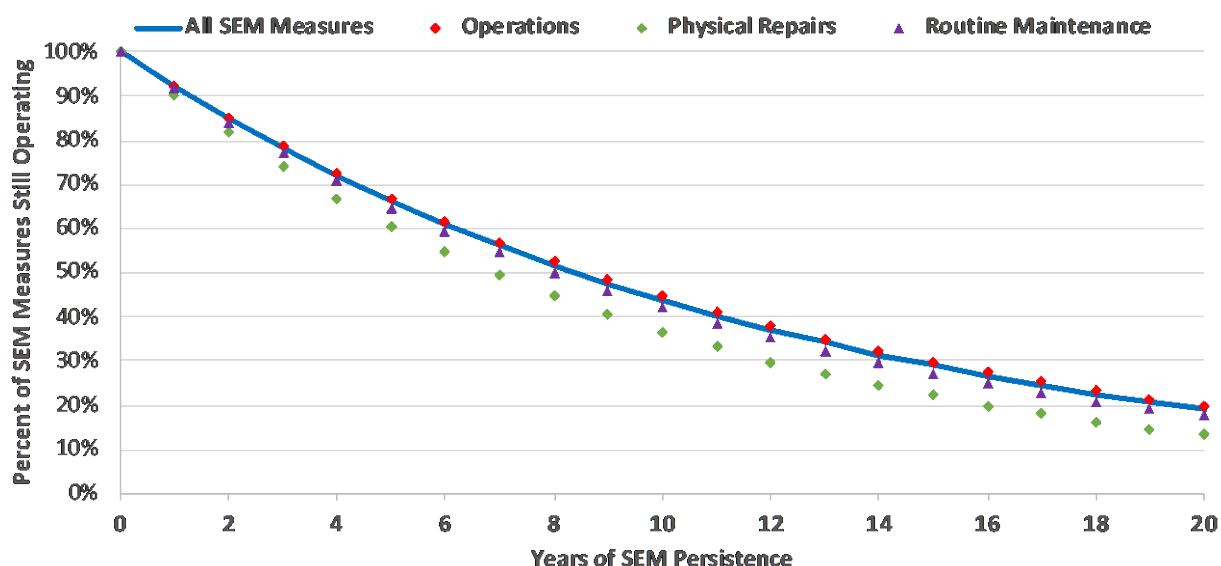
Figure 1: Smoothed survival curves for SEM measures
