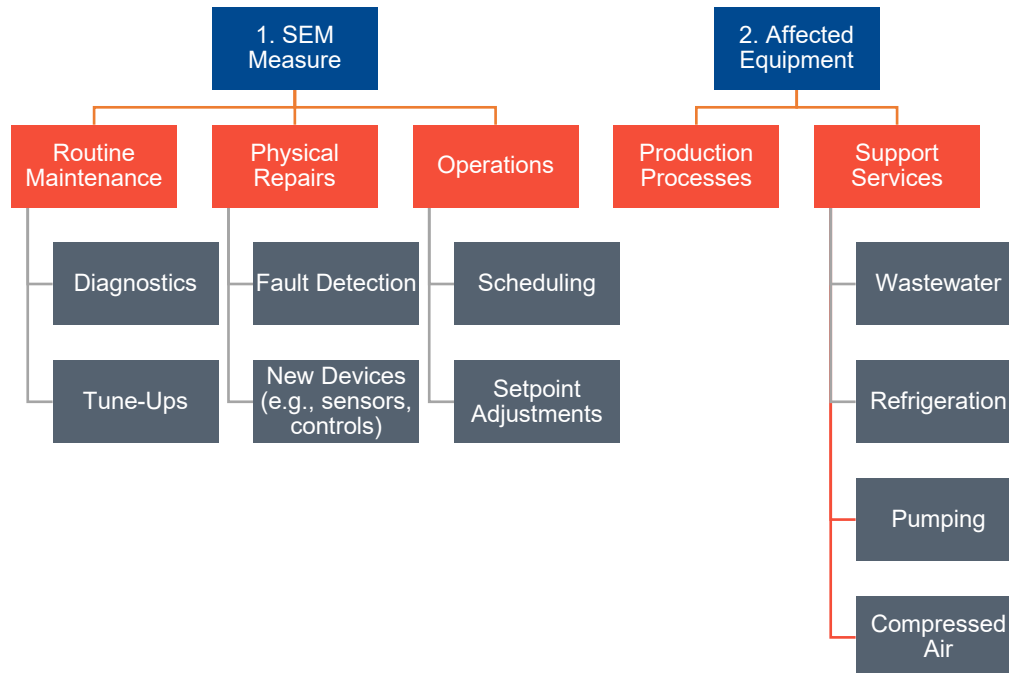
Figure 2: SEM Change classification framework
