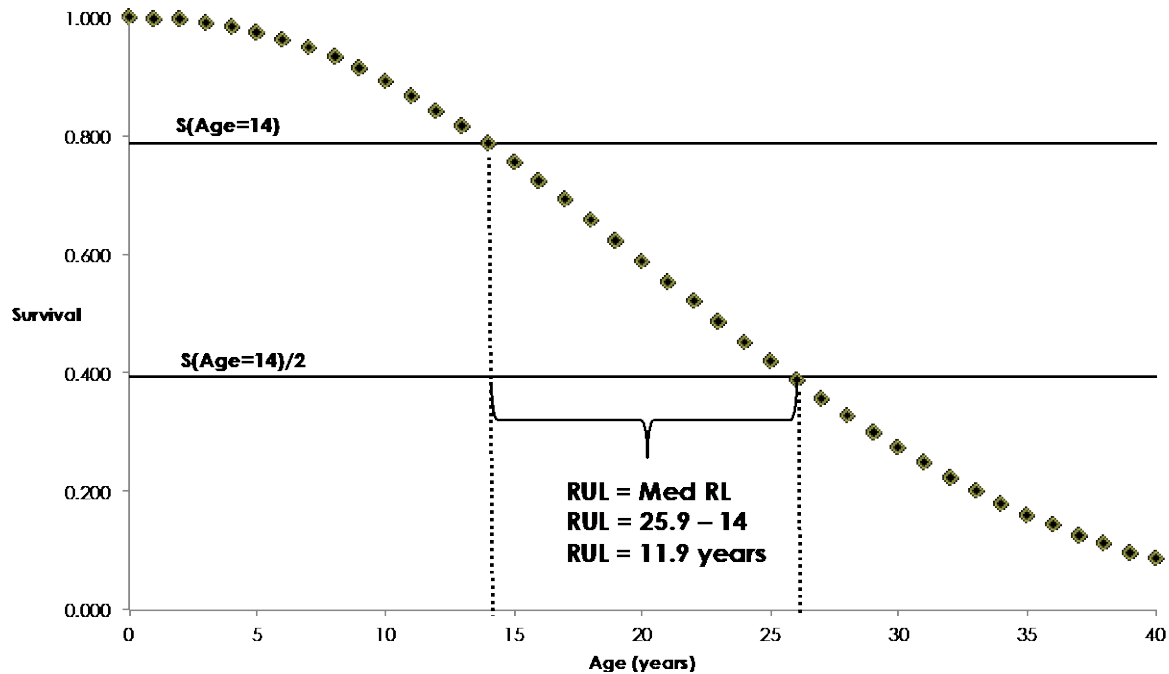
Figure 4: Computing median residual life based on a survival curve
