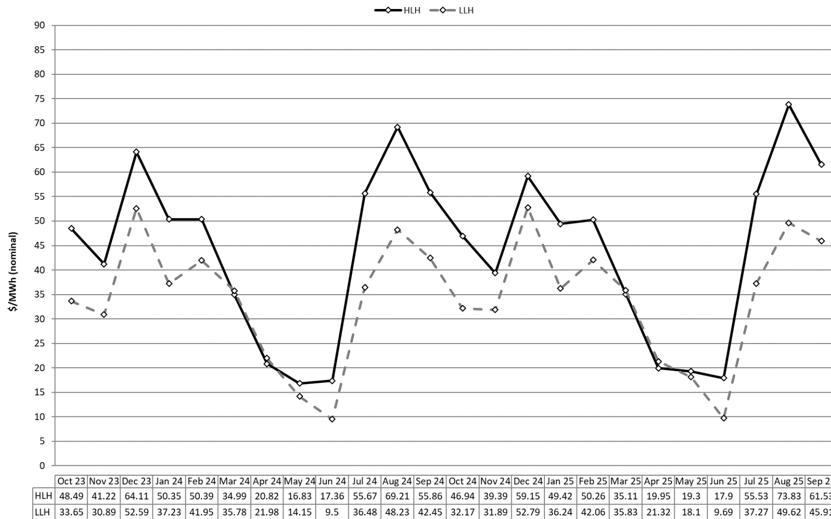
Figure 4: Monthly Average Mid-C Market Price for FY 24/FY 25 30 Water Years
