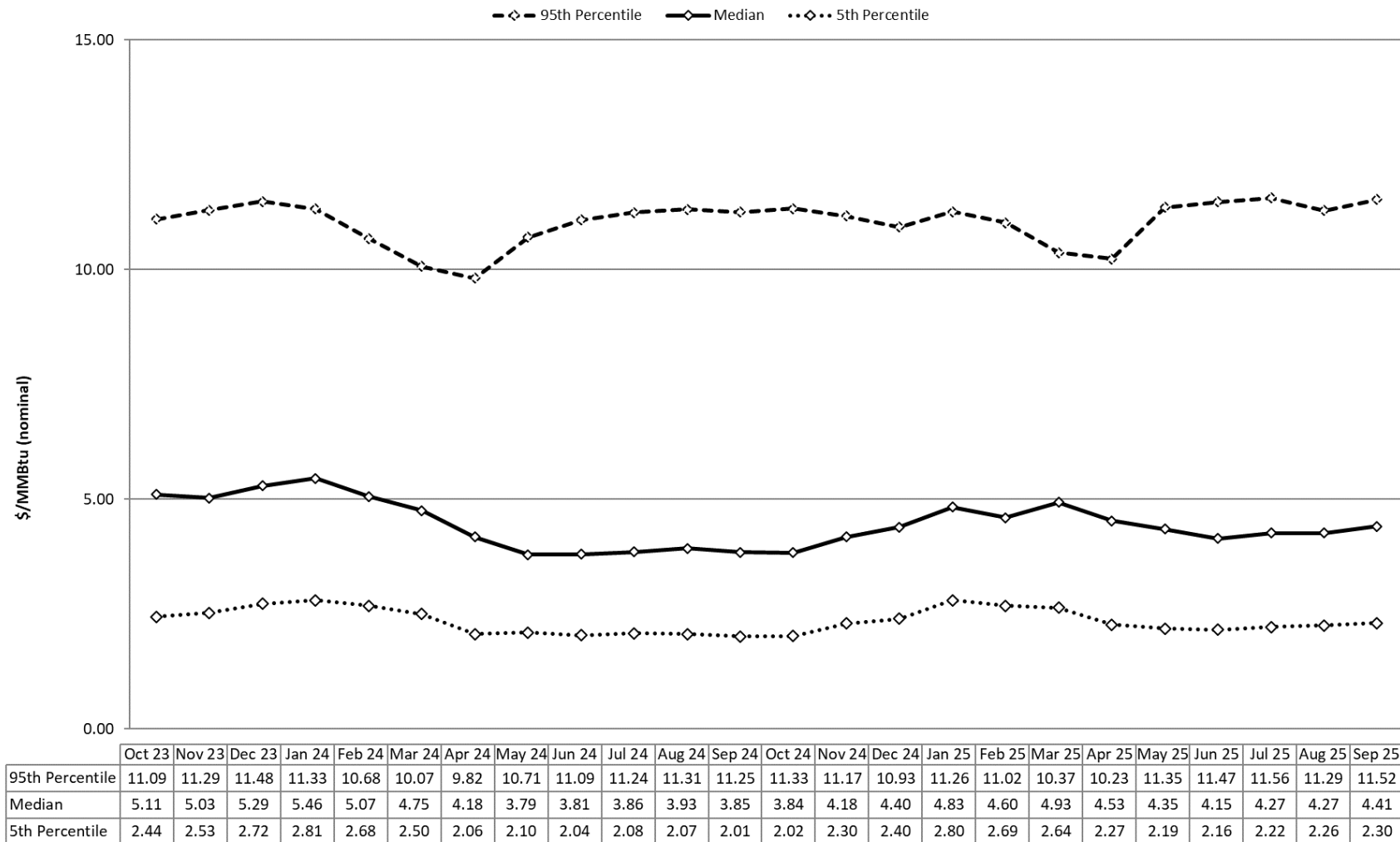
Figure 2: Natural Gas Price Risk Model Henry Hub Percentiles (Nominal $/MMBtu)
