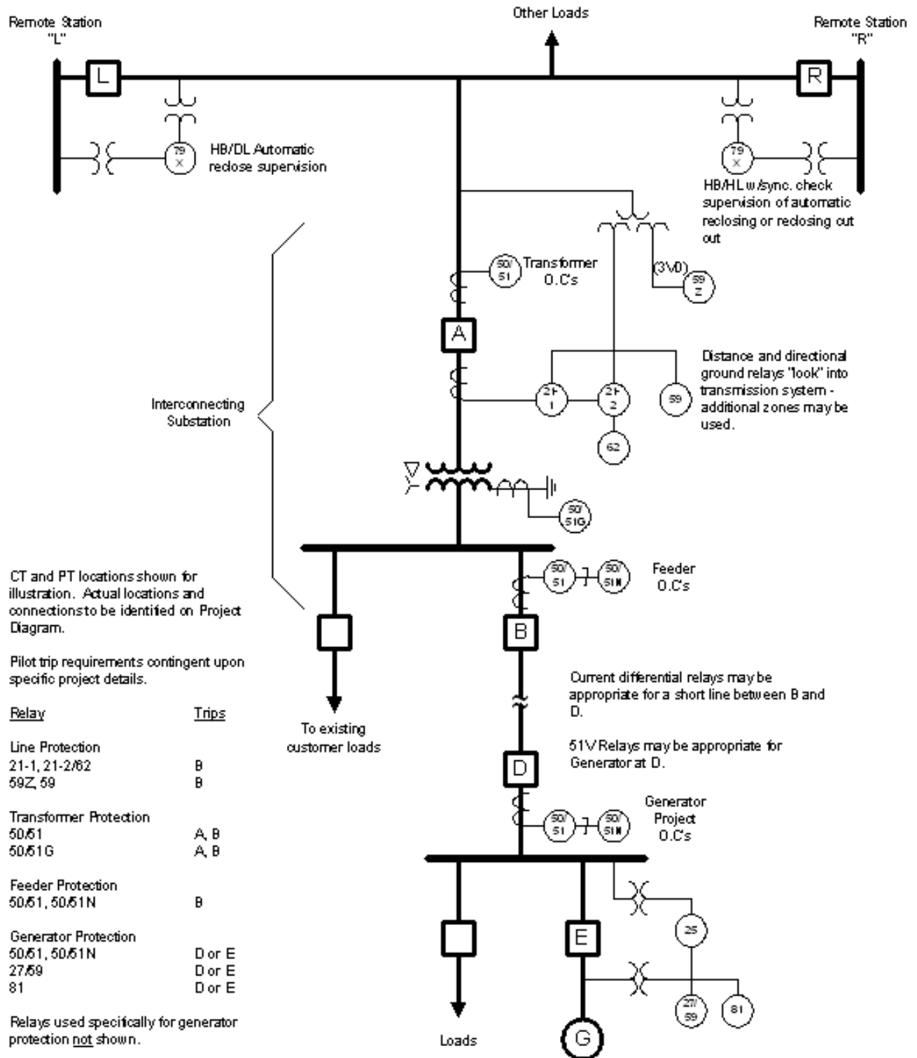
Figure 1212.--- Integration of Generation to an Existing Low Voltage Substation Connected to a Transmission line a \Delta -YG Transformer and Protected by a High Side Circuit Breaker (Switcher)
