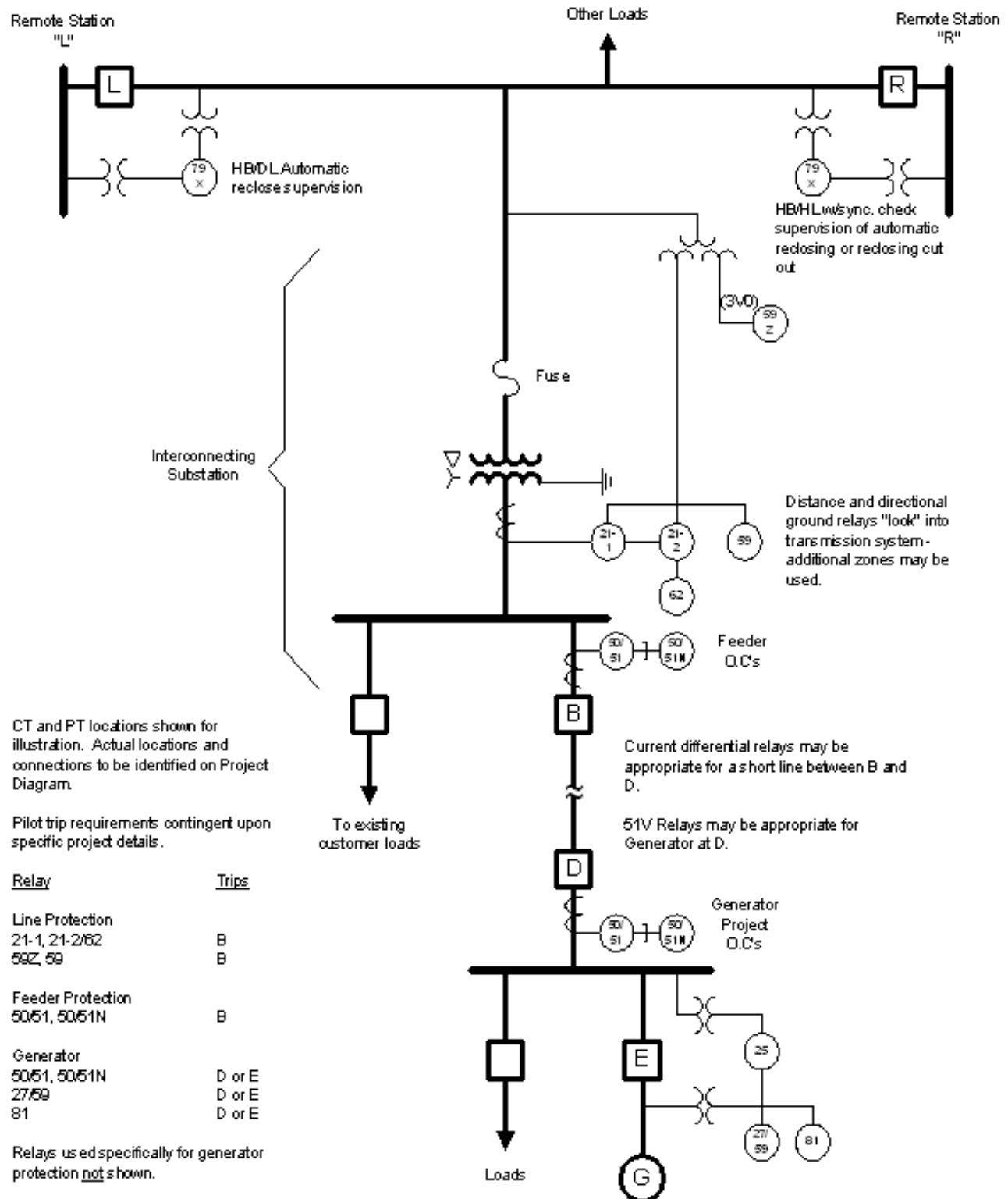
Figure 1111.--- Integration of Generation to an Existing Low Voltage Substation Connected to the Transmission line Through a Fused Δ-YG Transformer
